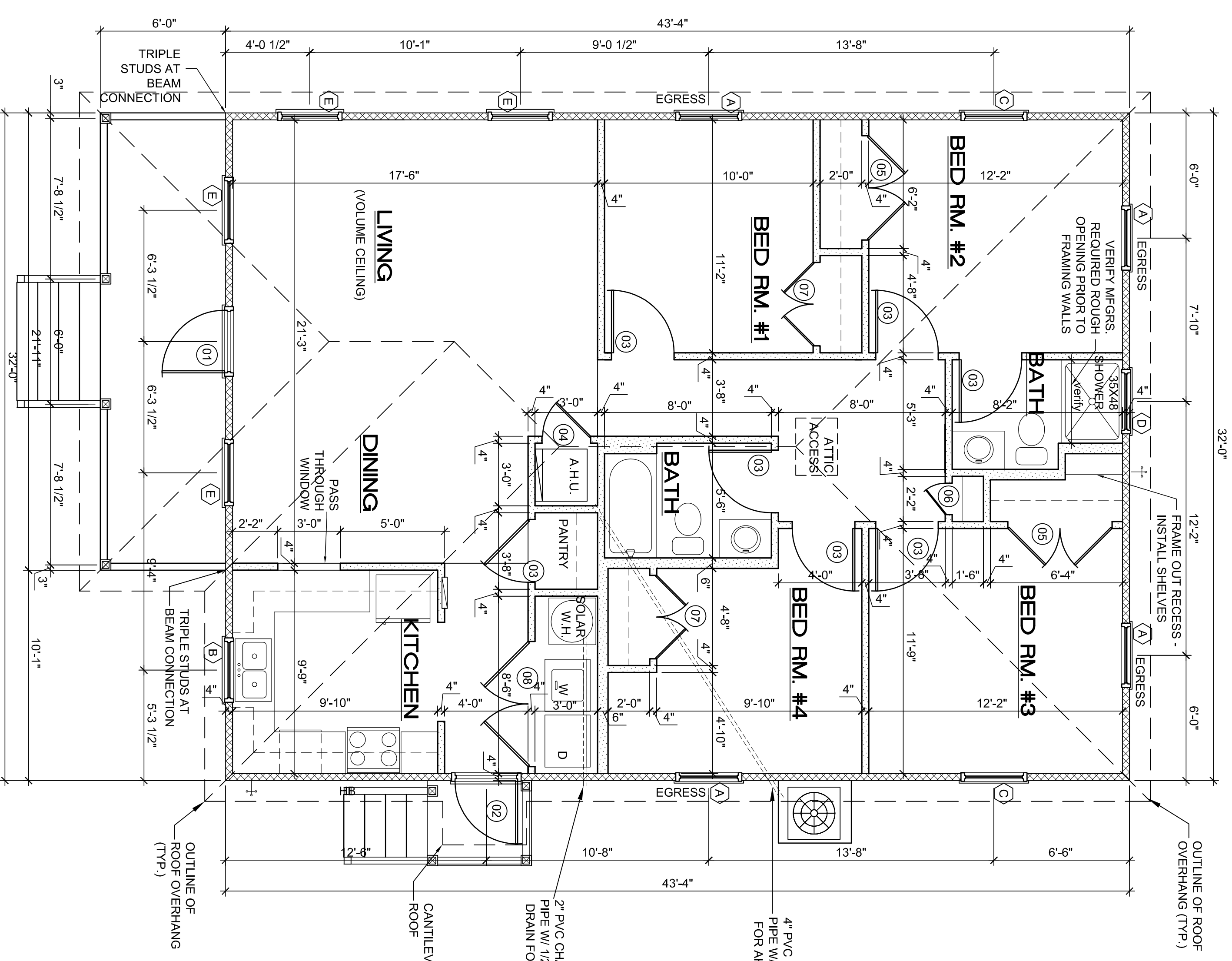
06 FLOOR PLAN SCALE: 1/4"=1'-0"
