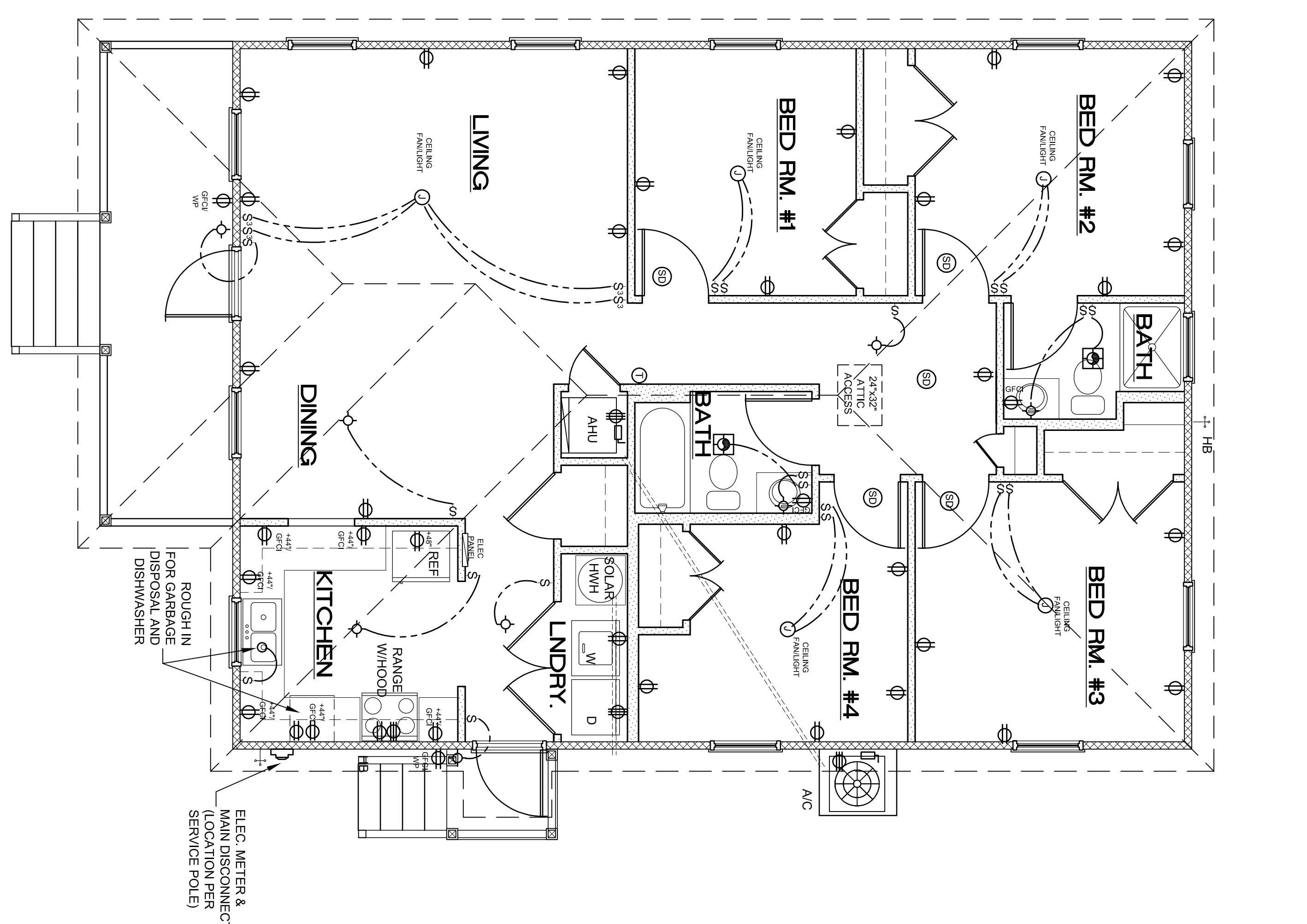
06 ELECTRICAL PLAN SCALE: 1/4"=1'-0"
